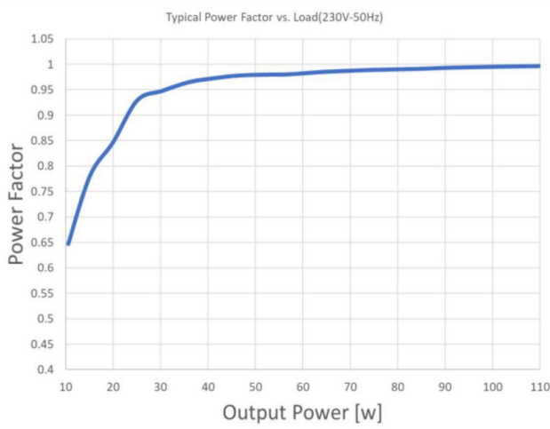
OT 110 0A7 NFC G3 Typical power factor vs Load
